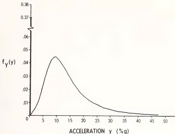
FIG. 3- DISTRIBUTION OF ACCELERATION, RISK ANALYSIS.
